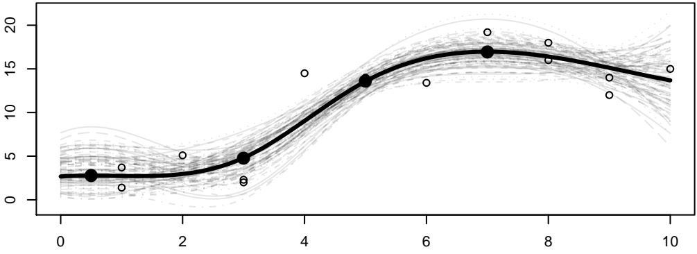
First derivative
