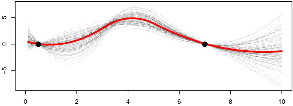
Second derivative
