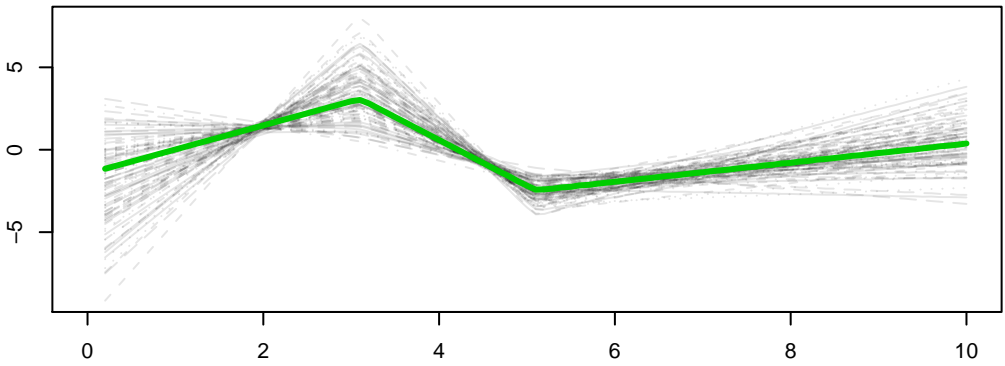
Third derivative
